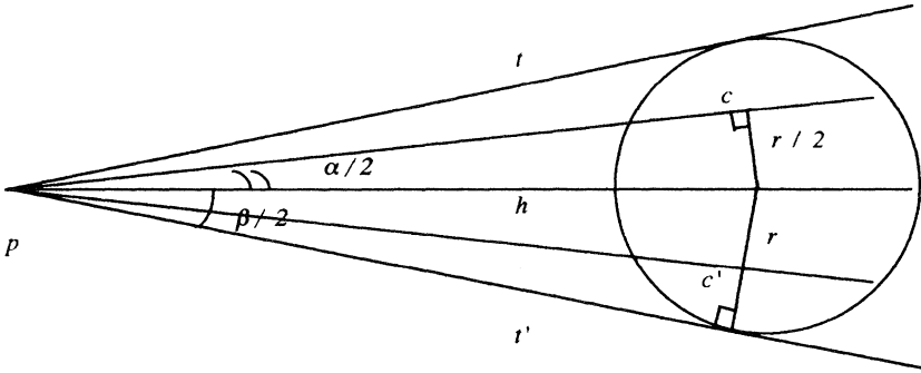
Figure 4.1. Solution to Q_2 (Classical Broom Straw Theory).
