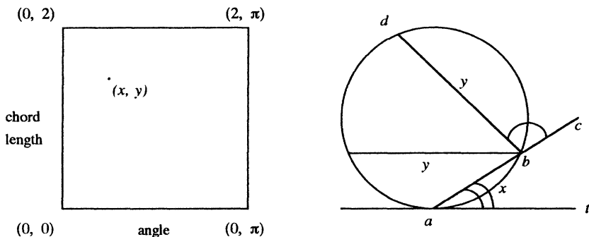
Figure 7.1. Randomizer Yielding Uniformly Distributed Chord Lengths.
